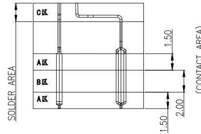
CONTACT PLATING DIAGRAM
