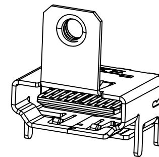
3D VIEWS
