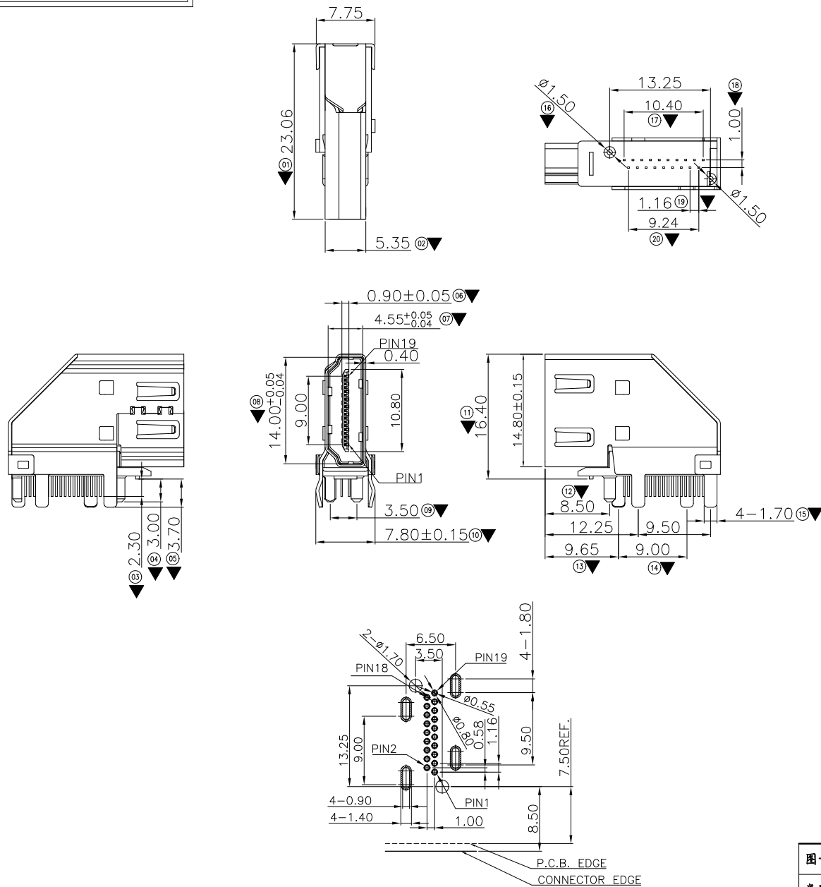
RECOMMENDED PCB LAYOUT (TOP VIEW) TOLERANCE: ±0.05mm
