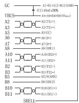
CIRCUIT DIAGRAM
