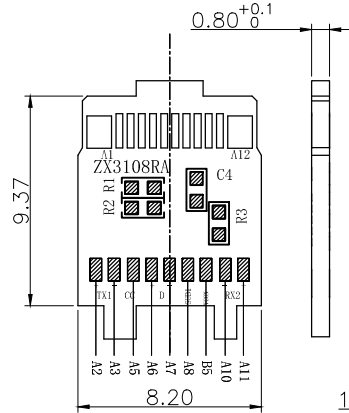
RECOMMENDED PCB LAYOUT TOP VIEW ALL TOLERANCE ±0.05
