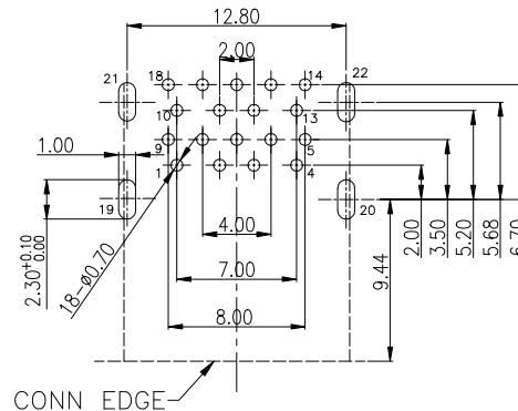
RECOMMENDED PCB LAYOUT TOP VIEW, TOL:±0.05MM
