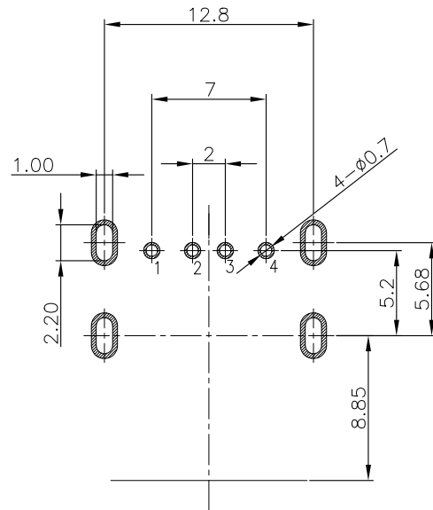
PCB LAYOUT(TOP VIEW T=1.60)
