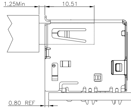
RECOMMENDED MOUNTING CONFIGURATION
